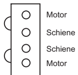
Stecker Motor/Schiene
